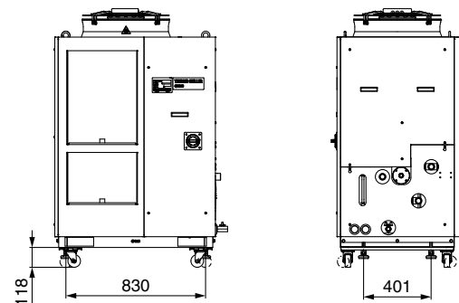
Fig. 1 Mounting view
