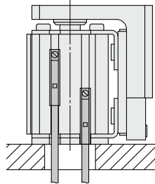
(3) When mounting the auto switch into the groove through the mounting surface.
